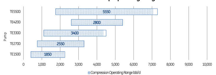
TE AR Modular Pump Operating Range
