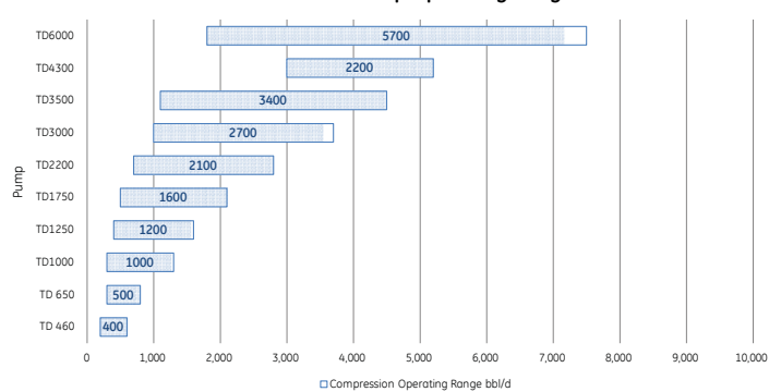
TD AR Modular Pump Operating Range
