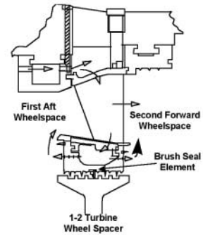
Proposed stage 2 nozzle design
