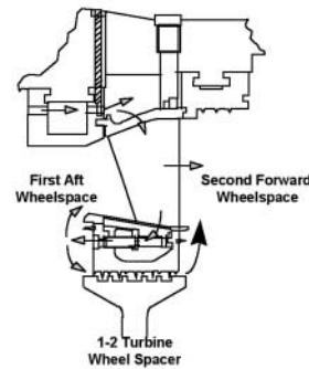
Current stage 2 nozzle design
